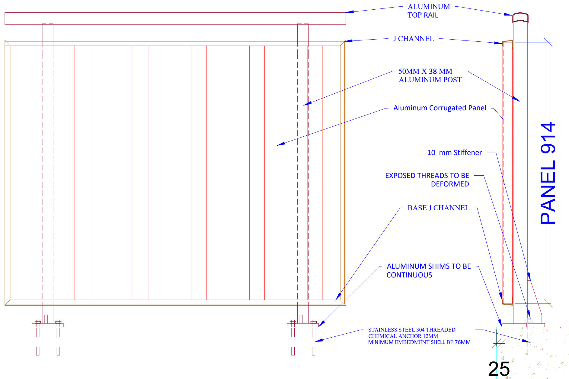
3 RAILING ELEVATION SCALE: NTS
