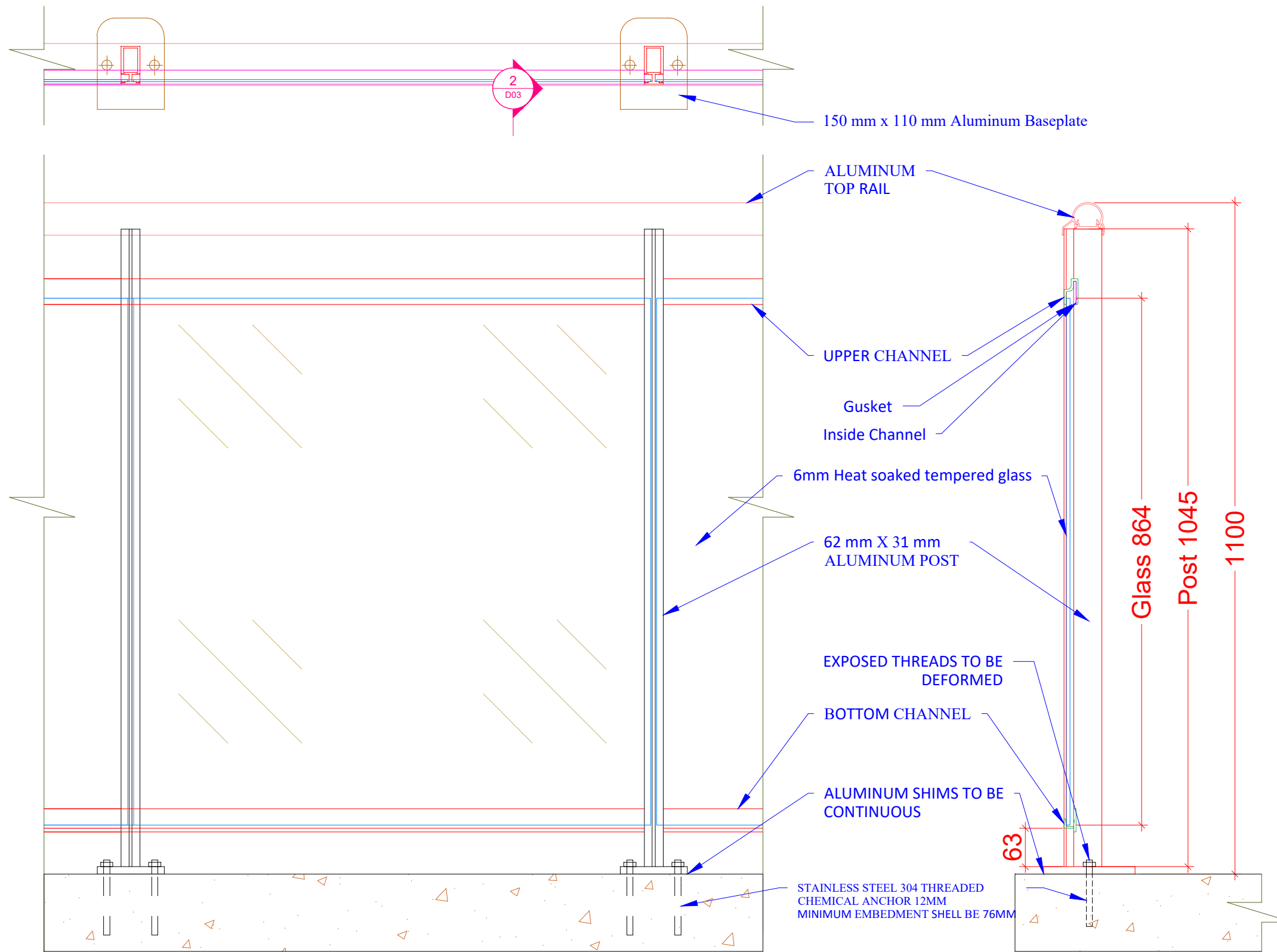
1 D03 GLASS RAILING SECTION DETAIL SCALE: NTS
