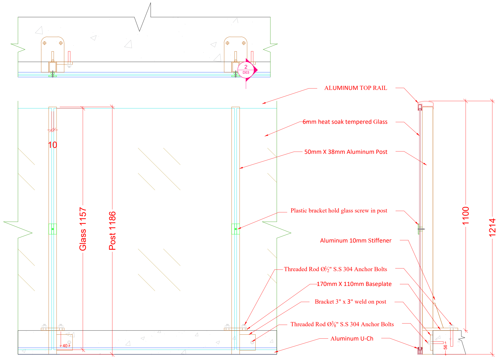
FRONT SIDE RAILING SECTION DETAIL
